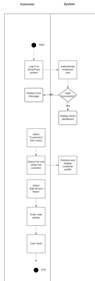
Activity Diagram for Record Driver's Notes
