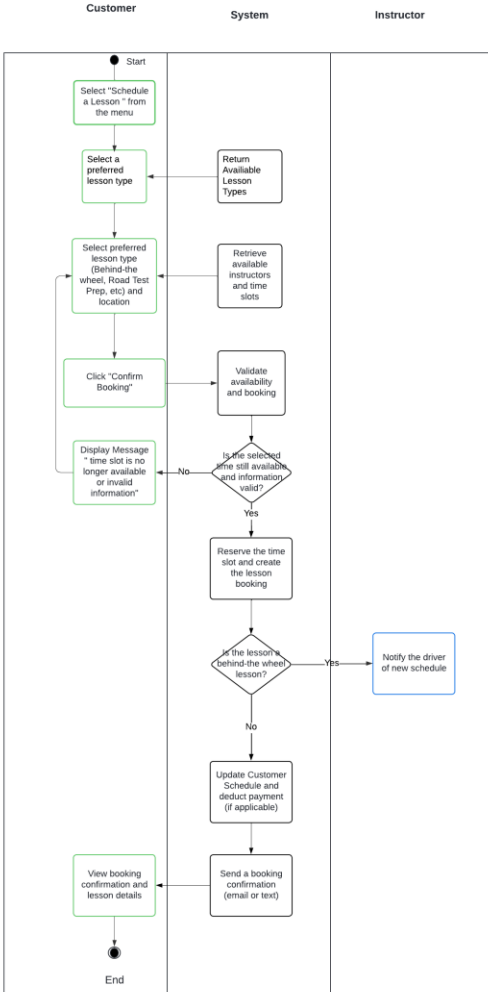
Activity Diagram for Schedule Driving Lesson
